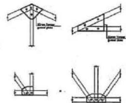
TRUSS CONNECTION DETAILS
