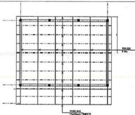
ROOF LAYOUT
