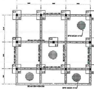
FOUNDATION LAYOUT 150mm thick slab
