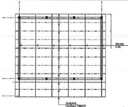
ROOF LAYOUT
